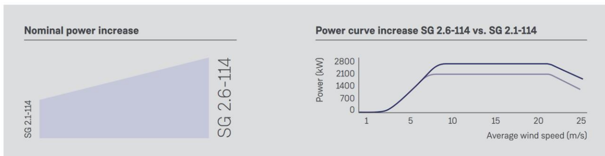
Figure 1.- 13% Nominal power increase of SG2.6-114 vs SG 2.1-114 model
